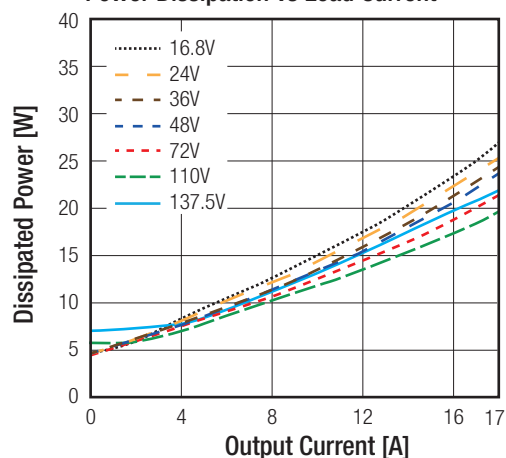
Power Dissipation vs Load Current
